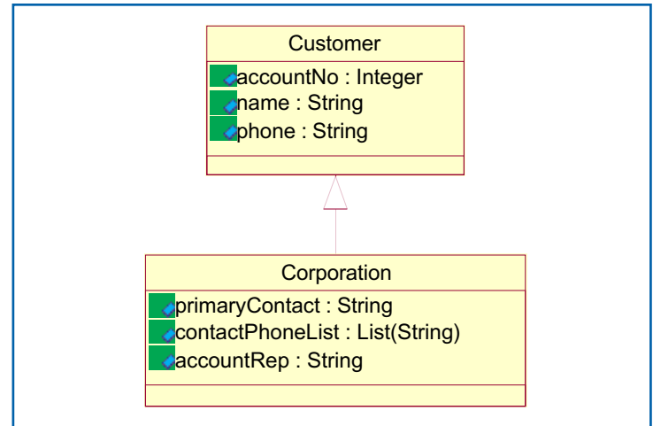
Figure 1: The class Customer and its subclass Corporation in UML
